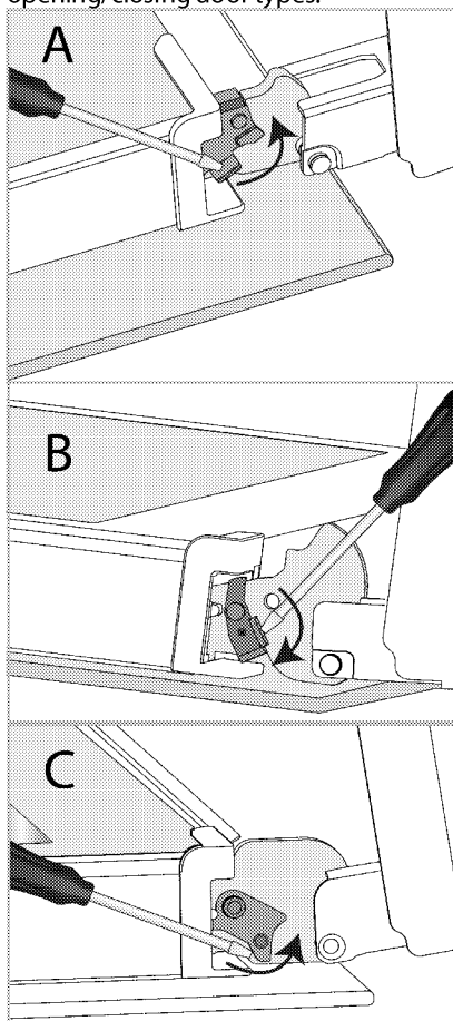
Hinge lock - closed position
